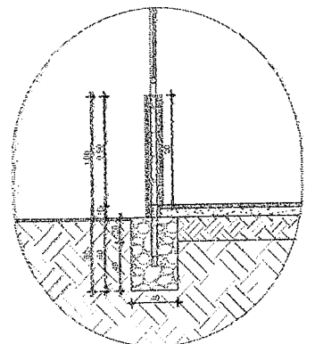
BASE ALAMBRADO 1M
